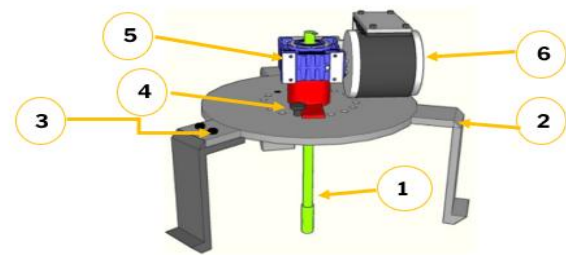
Gambar 2. Desain alat Automatic Speed Handle
